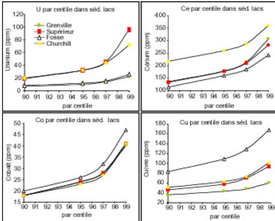
Figure 34: Lake sediment geochemical data were divided into subsets for each geological province. Anomalies are based on percentile thresholds. Here, element concentration vs. percentile plots are shown for U, Ce, Co and Cu in the Superior, Grenville, Labrador Trough and Churchill provinces. Return to the text.
