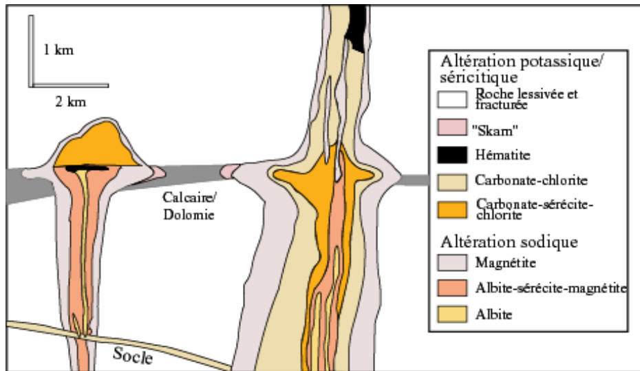
Figure 9: Hydrothermal alteration around iron oxide ore bodies depends on the depth of formation as well as the nature of the host rocks. The main alteration types are sodic (including disseminated magnetite) and potassic. The diagram shown here (after Hitzman et al., 1992) applies to an IOCG deposit in a sedimentary environment. Alteration would introduce about 5-9% K_2O and 5-8% Na_2O into the system. Return to the text.
