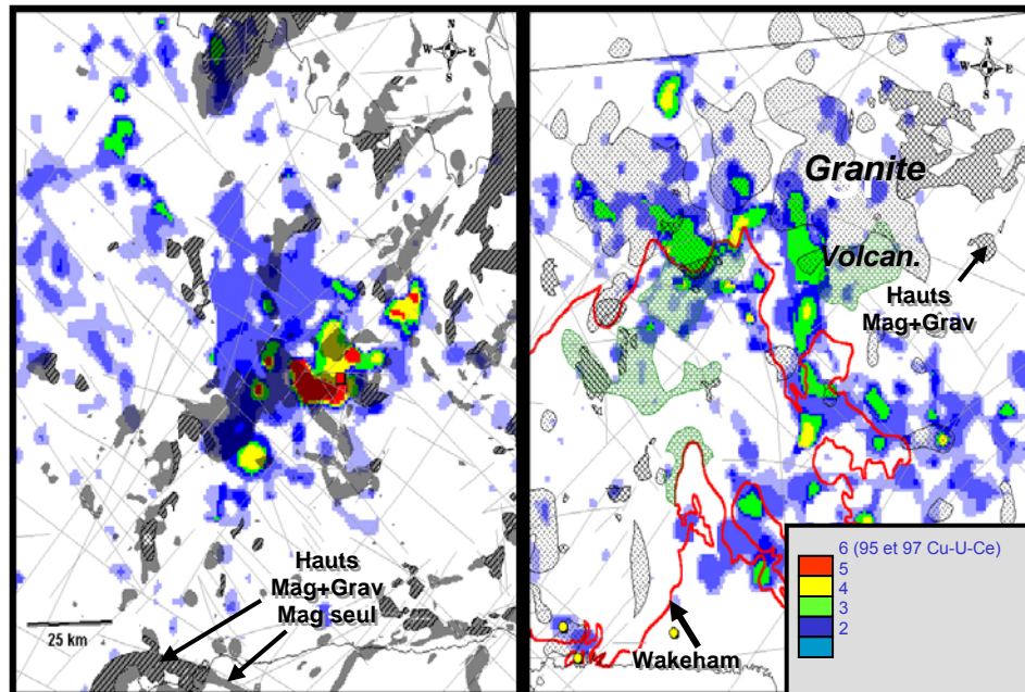
Figure 44: Close-up views of figure 43, showing the combination of geochemical and geophysical targeting approaches. Cross-hatching corresponds to coincident magnetic and gravimetric anomalies. On the left, Kwjibio is shown by a red square. Geochemical anomalies in this area are located at the intersection of NE-SW and NW-SE lineaments, or bounded by lineaments from these families. The areas where hot colors (geochemical anomalies) and cross-hatching (geophysical anomalies) are superimposed are the most favorable sectors for IOCG exploration. Return to the text.
