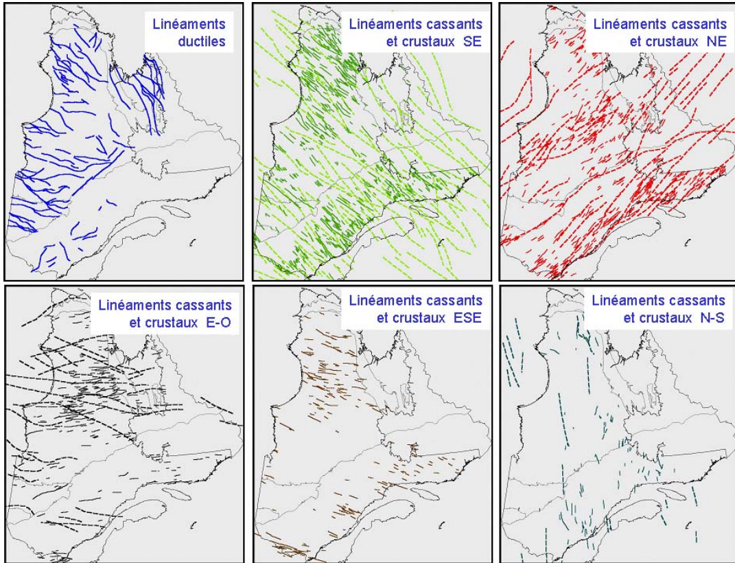
Figure 24: This figure illustrates the second method of subdividing geophysical lineaments into families using directional filters. The upper-left image contains all drag lineaments whereas sharp and crustal lineaments are spread into five groups over the other images. Drag lineaments are mainly found in the Superior Province and mostly have NW-SE orientations, although an E-W trend is also observed. They correspond to important deformation corridors (e.g., the Porcupine-Destor fault in the Abitibi subprovince). The most common orientation for sharp and crustal lineaments is NW-SE; many of these might be related to the opening of the Iapetus ocean. Return to the text.
