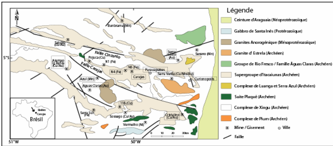
Figure 16: Salobo and neighbouring deposits in Brazil are the only Archean IOCG occurrences currently known. This geologic map of the Carajás mining district shows Salobo's location as well as other deposit types in the area (after Requía et al., 2003). Return to the text.
