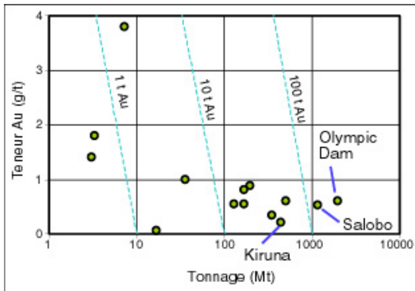
Figure 4: Most IOCG deposits contain 0.5 to 1.0 g/t Au (comparable to grades in porphyry gold deposits), but smaller IOCG occurrences can be richer in gold. Return to the text.
