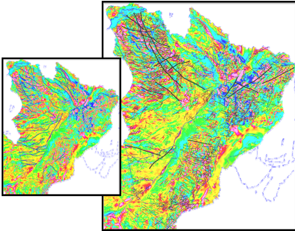
Figure 20: As most iron oxide deposits are structure-controlled, exploration can benefit from the identification of geophysical lineaments. These were obtained from the gravimetric (vertical gradient) and magnetic (total field) maps. Three types of lineaments have been distinguished: (1) sharp lineaments, which are interpreted as brittle faults; (2) drag lineaments, which are characterized by folding and drag of the magnetic grain near magnetic lows which are continuous and parallel to the tectonic grain; these are interpreted as ductile deformation corridors; and (3) crustal lineaments, which separate distinct gravimetric domains. Both maps here display the magnetic field; on the left, drag lineaments are shown as blue lines (n = 98); on the right, sharp lineaments are shown as black lines (n = 1913). Wider lines correspond to lineaments 200 km long or more. Return to the text.
