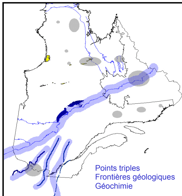
Figure 51: Compilation map of the favourable areas for iron oxide exploration in Quebec. These areas correspond to triple junctions, deformation zones at subprovince boundaries, or isolated geochemical anomalies. Return to the text.
