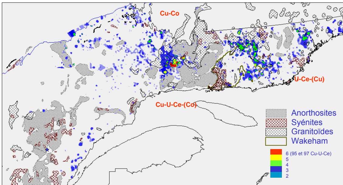
Figure 43: Grenville province, fuzzy logic method for lake-bottom sediment geochemical anomalies. A value of one is given to each pixel having Cu, Ce or U concentrations above the 95 th and the 97 th percentile, for a possible maximum value of six. Rock types favourable for iron oxide exploration are shown as well. The greatest anomalies are found NE of Sept-Iles, in the Kwijibo area. Most sectors displaying fuzzy logic totals \geq 4 are found either within or near granitoids, or at the northern and eastern margins of the Wakeham Group (red rectangle on the right). Return to the text.
