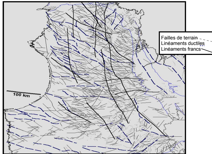
Figure 22: Comparison of the pre-2001 observed and interpreted faults (provincial government data) with the sharp geophysical lineaments determined in this study. Return to the text.
