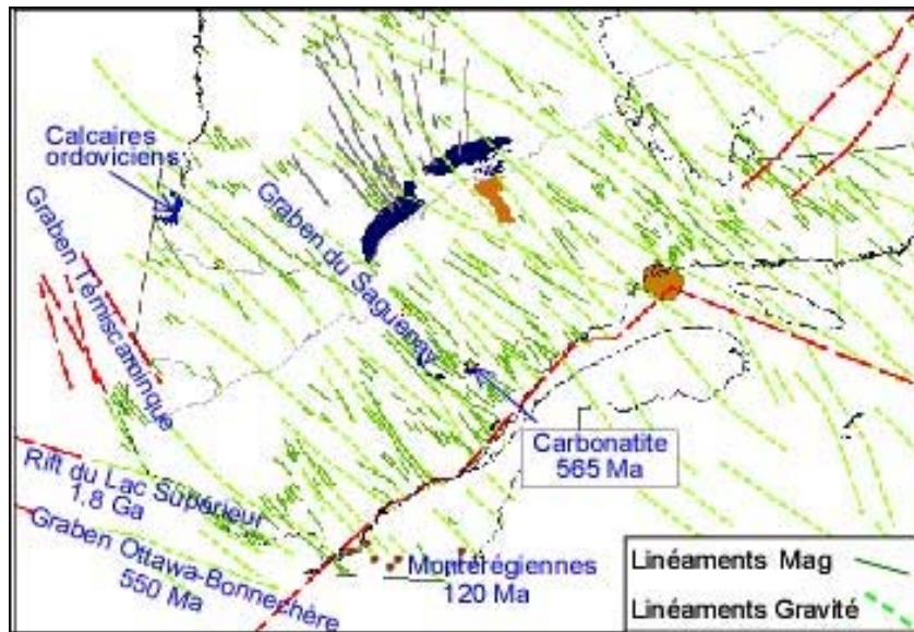
Figure 25: Here the NW-SE lineaments are divided by origin: gravimetric (pale green lines) or magnetic (darker green). Also shown are various failed rifts or grabens. In the southern part of the Mt-Laurier basin (Grenville Province), Fe-U mineralization lies at the intersection of the early Proterozoic Lake Superior rift and the Mesozoic Timiskaming graben. Similarly, Fe-apatite deposits in the Adirondack lie at the intersection of two extensional structures. Return to the text.
