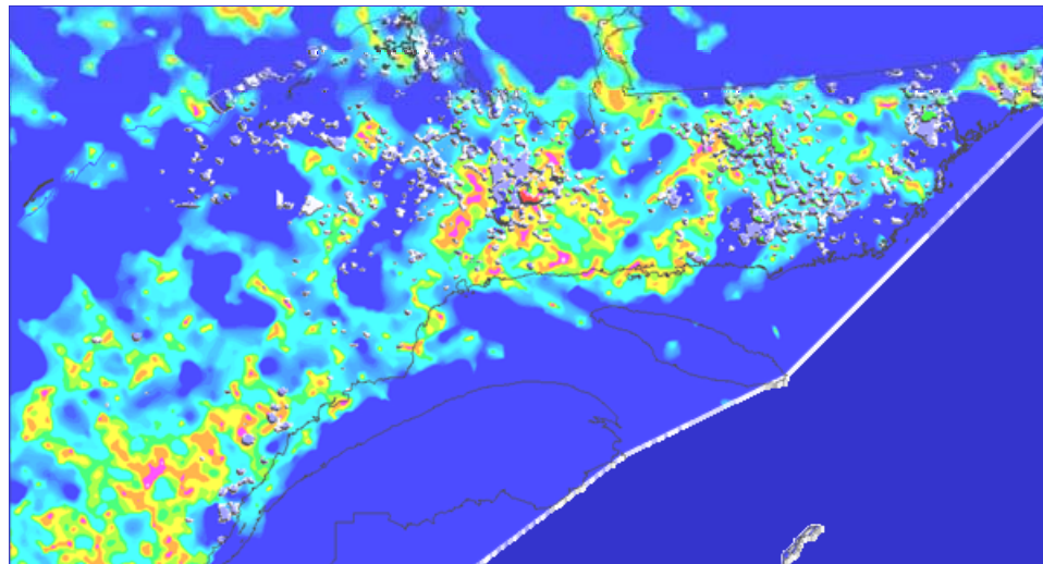
Figure 45: Combined geochemical and structural approaches for the Grenville Province. The density of geochemical anomalies is shown by shades of grey; the density of lineaments is shown by a colour scale from blue to red. Return to the text.
