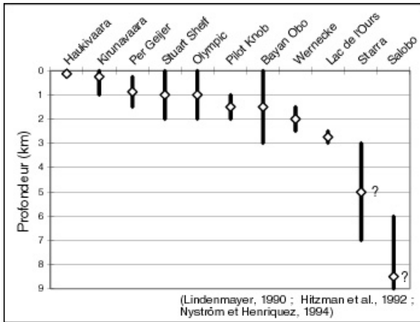
Figure 8: Most iron oxide deposits are thought to have formed at depths of 2 km or less, given the presence of brittle structures, open space-filling textures, associated volcanism, etc. However, Starra in the Cloncurry district (Australia), and Salobo in Brazil could have formed deeper, although the exact depths are unknown. On this diagram, the lozenges show the inferred depths of formation for various deposits, with error bars. Return to the text.
