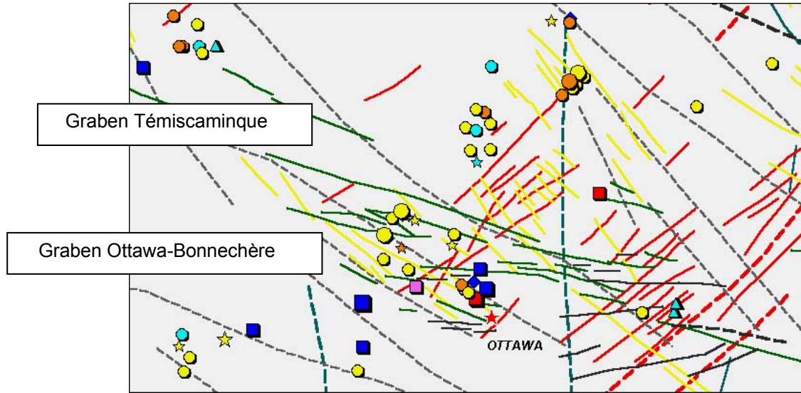
Figure 38: Map of southern Quebec and part of Ontario showing magnetic lineaments (lines coloured by orientation) and gravity lineaments (dashed lines). The location of the known iron oxide deposits (and related mineralization), from figure 36 (with identical symbolism) is superimposed. Many U occurrences (yellow dots) west of Ottawa, and a few north of the Mt-Laurier basin, are located near or within coincident magnetic and gravimetric anomalies. Return to the text.
