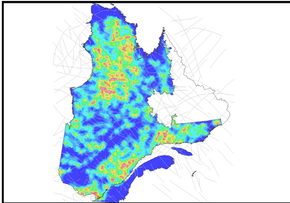
Figure 29: To evaluate the density of lineaments, they were segmented into a series of aligned points. The density of these points is shown in a grid; here the low densities are in blue and the high densities in red. Return to the text.
