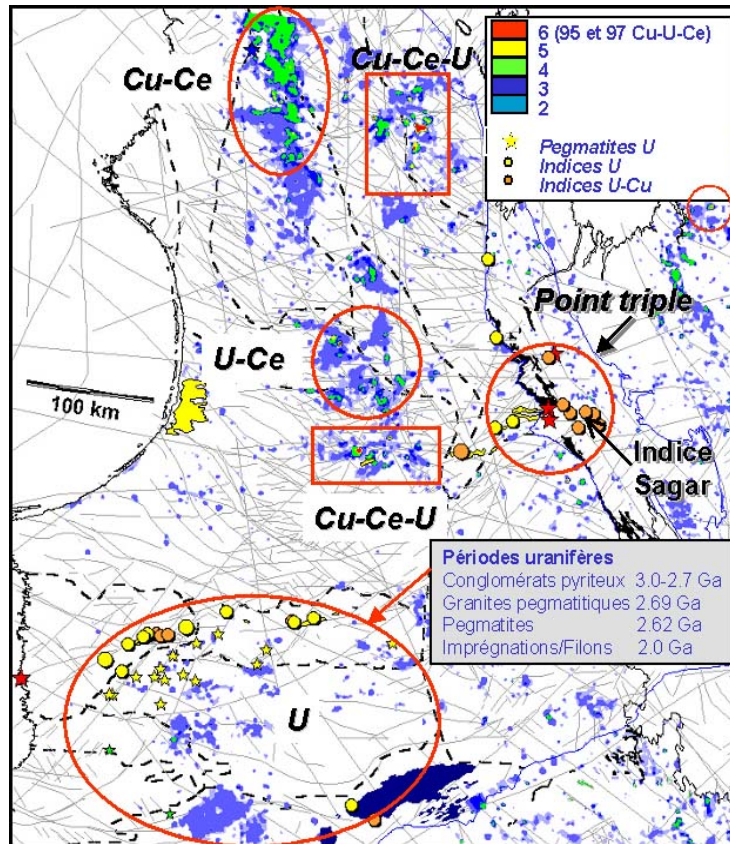
Figure 49: Regional exploration targets in the Superior province, using fuzzy logic on lake-bottom sediment geochemical anomalies. A value of one is given to each pixel having Cu, Ce or U concentrations above the 95 th and the 97 th percentile, for a possible maximum value of six. Known uranium and U-Cu showings were added, as well as interpreted geophysical lineaments. The red rectangles are examined in more detail in the next figure. Return to the text.
