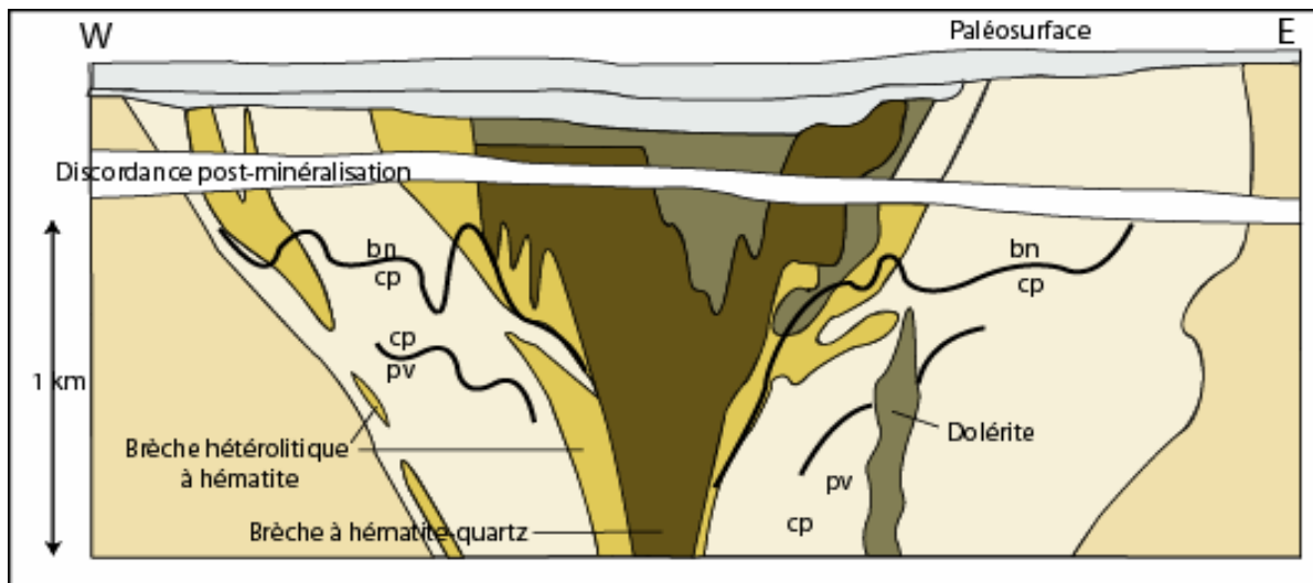
Figure 6: The shape of iron oxide deposits is complex; it is often controlled by permeable zones along either faults, favourable horizons, or intrusive contacts. Discordant mineralized bodies result from injections and cross-cut the stratigraphy as breccia bodies, pipes, dikes, veins or irregular masses. Such systems can reach 1 km vertically. This figure shows an E-W cross-section through Olympic Dam, the best-known discordant IOCG deposit (after Hitzman et al., 1992). Return to the text.
