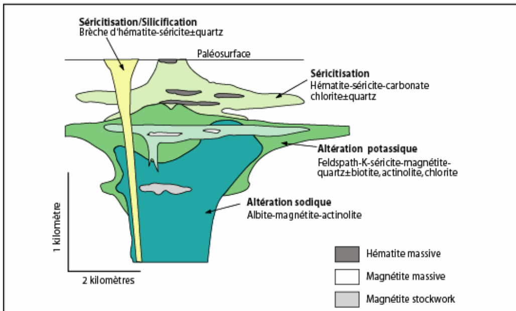
Figure 10: Another hydrothermal alteration zonation diagram after Hitzman et al. (1992). This one applies to IOCG deposits in volcanic or plutonic rocks. Return to the text.
