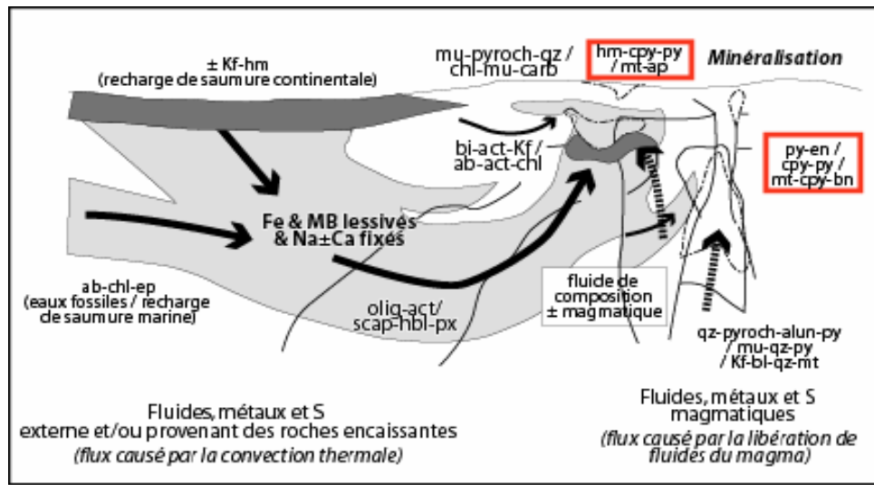
Figure 15: Given that the nature of magmatism is very variable around iron oxide deposits, and that deposits such as those of the Cloncurry district have no link with intrusions, it has been suggested that the large hydrothermal systems accompanying iron oxide deposits might not have a magmatic origin. Sulphur-poor briny solutions could be important for the transport of Na, Fe and base metals. Figure after Barton and Johnson (2000). Return to the text.
