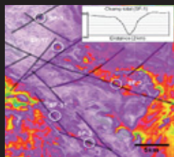
TYPICAL MAGNETIC SIGNATURE ASSOCIATED WITH KIMBERLITE
